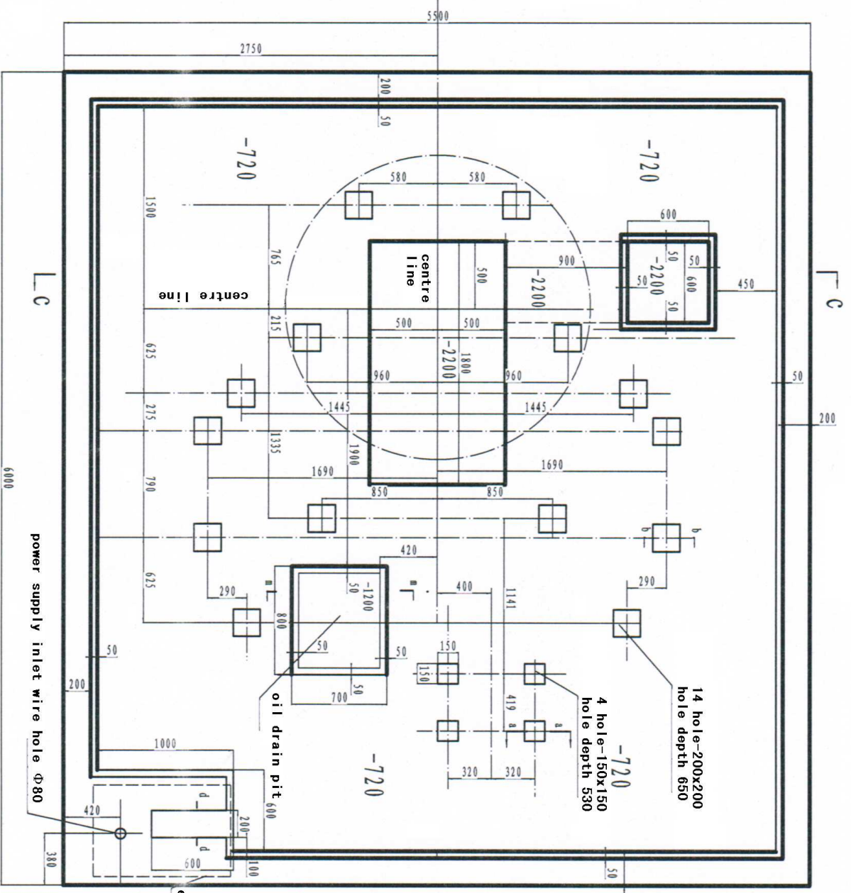
C5225 foundation drawing
